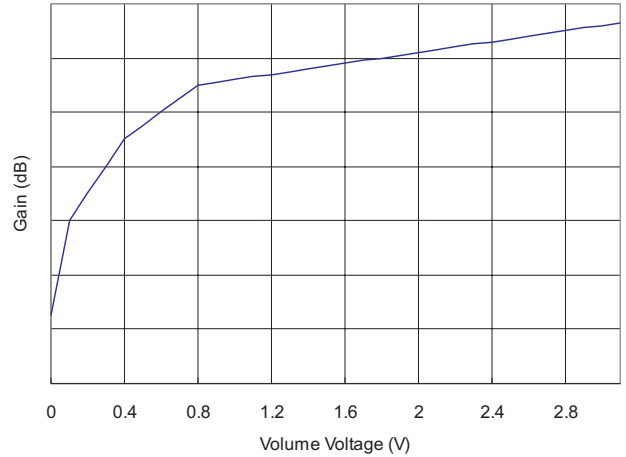
21. Gain vs DC voltage
