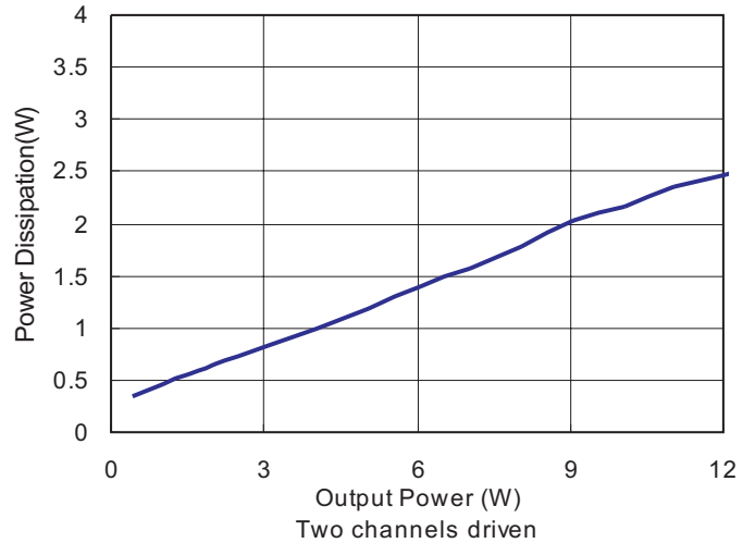
22. Power Dissipation vs. Output Power
